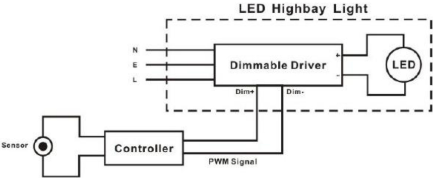
Schematic Circuit Diagram
