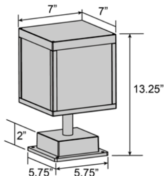
Line Drawing #1
