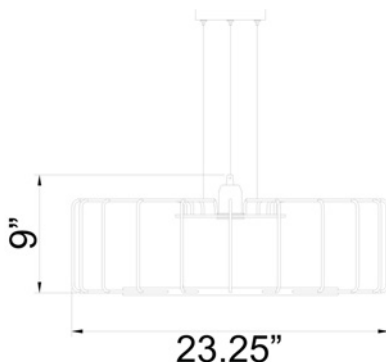
Line Drawing #1
