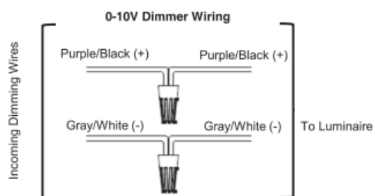
Wiring Diagram 2
