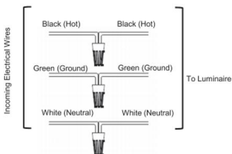
Wiring Diagram 1
