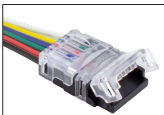
HD Power Feed (6-wire) TL-6PWR-HD
