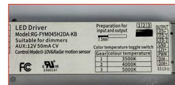
SWITCH CCT SELECTABLE
