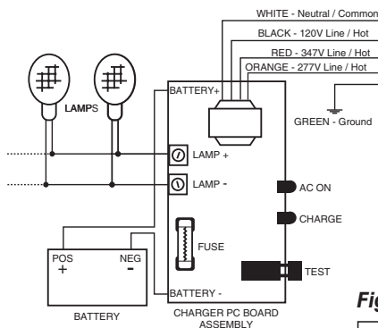
Figure 3 CHARGER BOARD STANDARD DUAL INPUT VERSION
