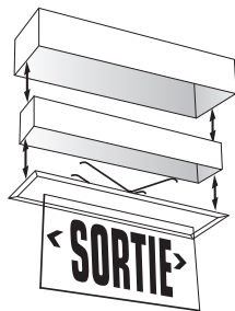
Trim and faceplate mount into backbox for quick and easy installation.
