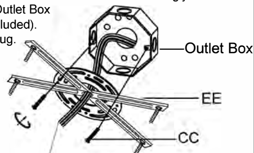
Supply Wires with Outlet Box Screws Ground Wire
