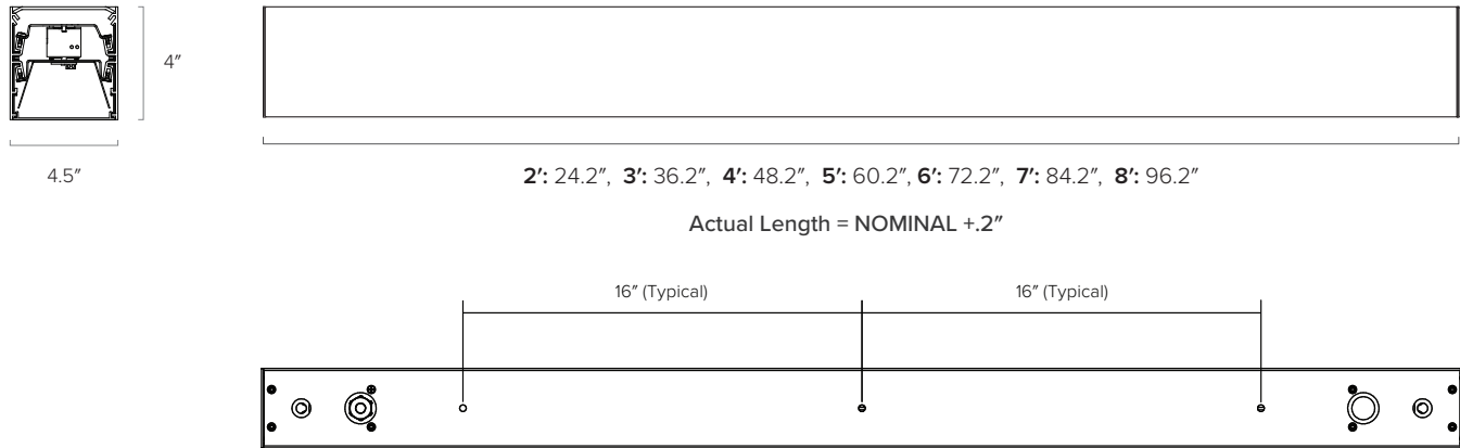
Mounting Locations - Single Unit
