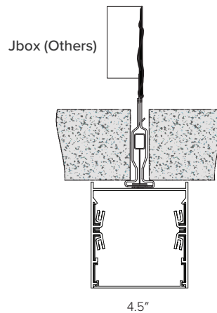
T-Bar 9/16" Aircraft Cable (ACY)
