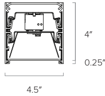
0.25" Regressed Lens
