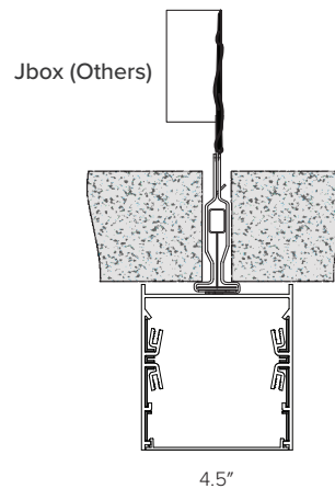
T-Bar 15/16" Aircraft Cable (ACY)
