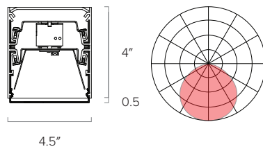
0.5" Drop Lens
