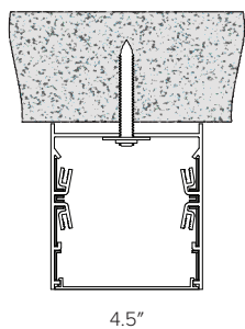
Solid Ceiling 1/4" - 20 Thread Required (1)
