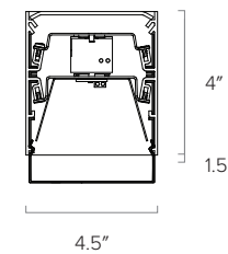
1.5" Drop Lens
