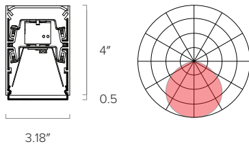
0.5" Drop Lens
