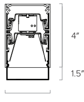
1.5" Drop Lens
