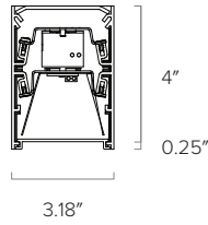
0.25" Regressed Lens
