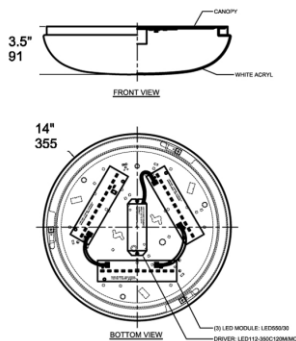
CL-T6113-6-LED03 Dimensions mm | 356(W) x 89(H) inch | 14(W) x 3.5(H)
