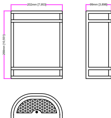
WS-A5422LED02-120 (Triac Dimmable)
