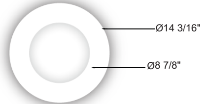
CDFPGoofRing109
