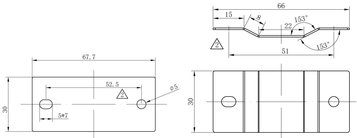
SWS-Connector
