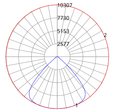
BAY-E-208/150W/8xx-U with optional field installed 90° lens
