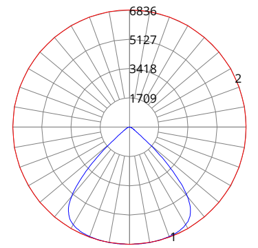
BAY-E-138/100W/8xx-U with optional field installed 90° lens
