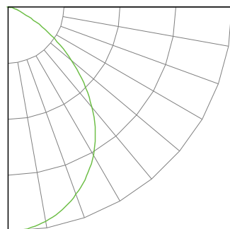
CD10/PS33/FCCT/UD (Typical performance @33W, 4000K)
