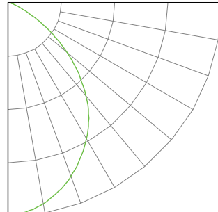
CD8/PS22/FCCT/UD (Typical performance @22W, 4000K)
