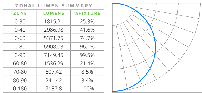
SCS/PS60/8xx/UD (Typical performance @4000K; Standard distribution)
