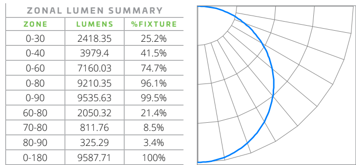
SCS/70W/8xx/UD (Typical performance @4000K; Standard distribution)
