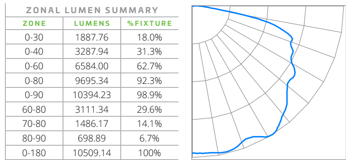
SCS/70W/8xx/UD/G (Typical performance @4000K with Garage distribution)*
