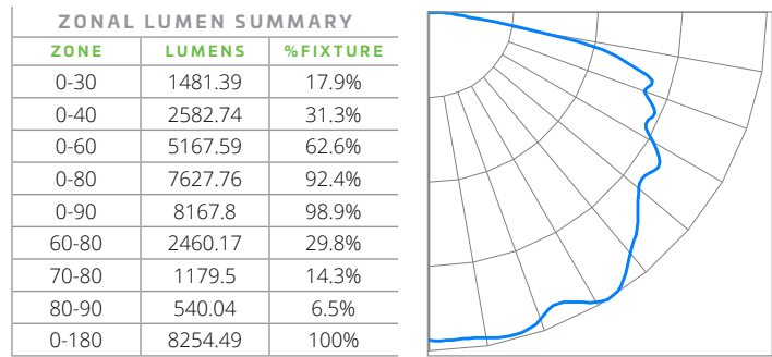
SCS/PS60/8xx/UD/G (Typical performance @4000K with Garage distribution)*
