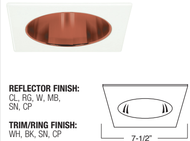
B687CP-WH SQUARE REFLECTOR TRIM
