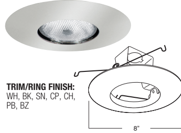
AF633CH R/PAR30 OPEN TRIM
