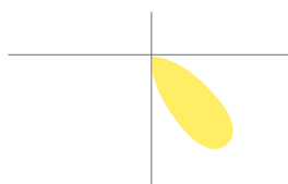
WALL WASH Candlepower Distribution Curve
