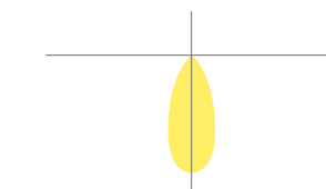
NS: NARROW SPOT Candlepower Distribution Curve
