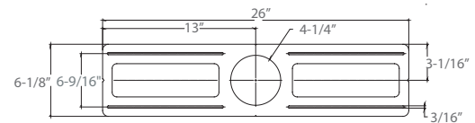
RL-ACC-SLIM-4-F-ROUGHPLATE Rough-in plate for use with 4" downlights
