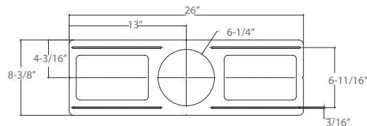
RL-ACC-SLIM-6-ROUGHPLATE Rough-in plate for use with 6" downlights
