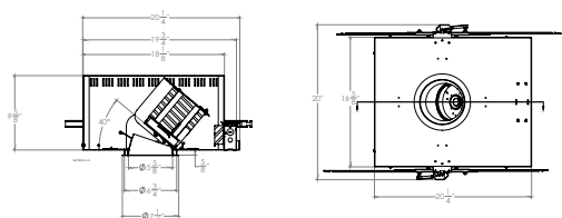
6000 Lumens Line Drawing
