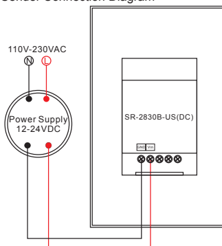
Sender Connection Diagram
