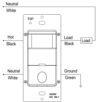
Wiring Diagram
