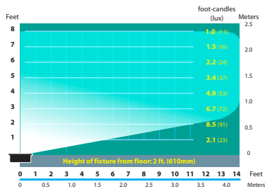
SL-08-FL-5 Half Spread Photometrics (5w)
