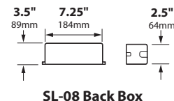
SL-08 Back Box
