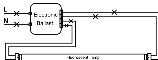
Programmed Start or Rapid Start Configuration
