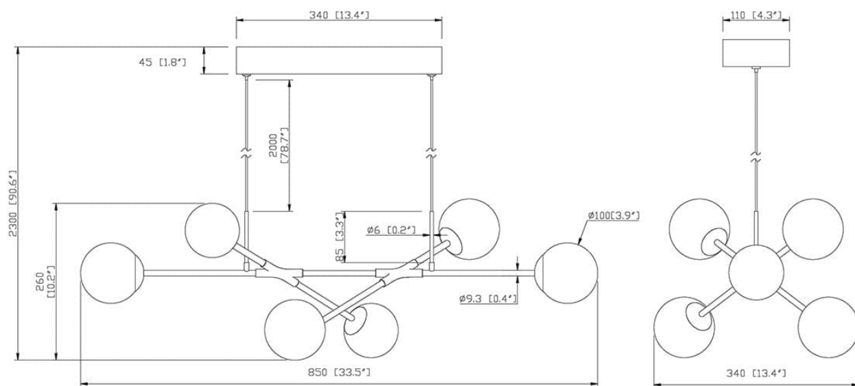
Model: PF211-6L-BLK/BRS
