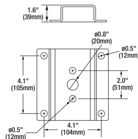
Wall Mount (60129 or 60652)
