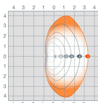
AREAFLD2A-240W-T5 at 45° tilt
