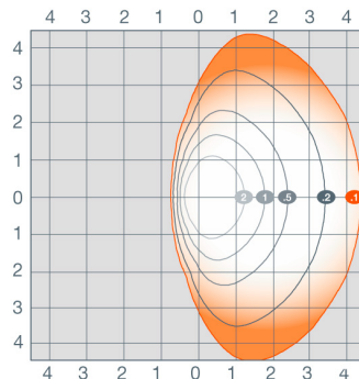
AREAFLD2A-240W-T3 at 45° tilt
