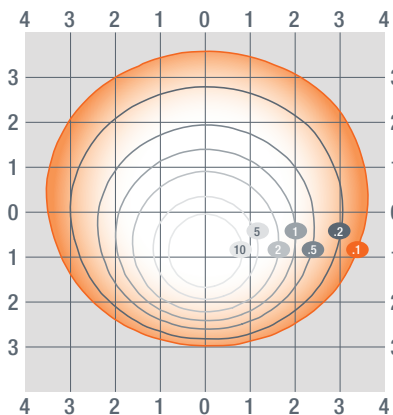
105W 15ft mtg height – 15 degree tilt
