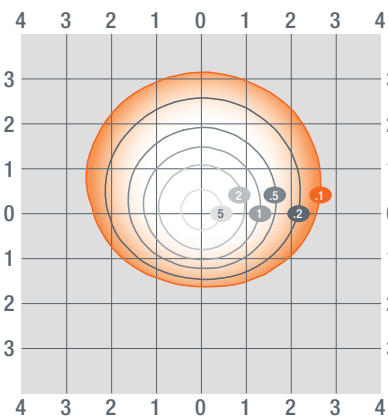
80W 15ft mtg height – 15 degree tilt
