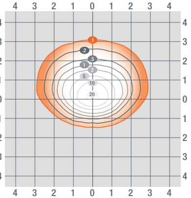
255W 25ft mtg height – 15 degree tilt
