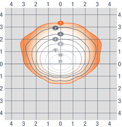
290W 25ft mtg height – 15 degree tilt
