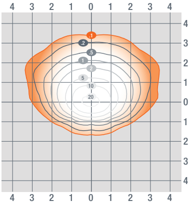
330W 25ft mtg height – 15 degree tilt
