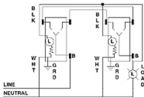
3-Way Pilot Light
