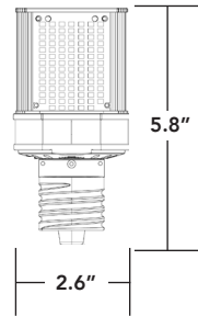
LED-8087M
