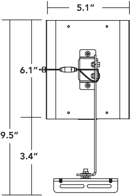
RPT-LEDBLOCK-150L/ RPT-LEDBLOCK-200L
