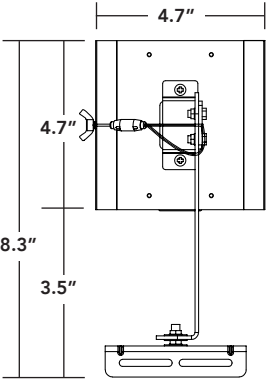
RPT-LEDBLOCK-65L/ RPT-LEDBLOCK-100L
