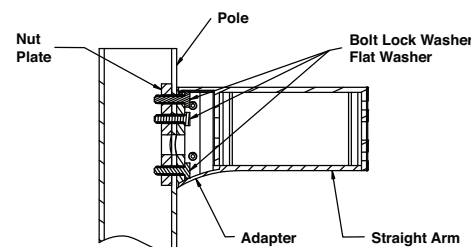
Sectional drawing of the pole and straight arm mounting
