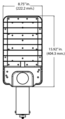
60/75W Model
