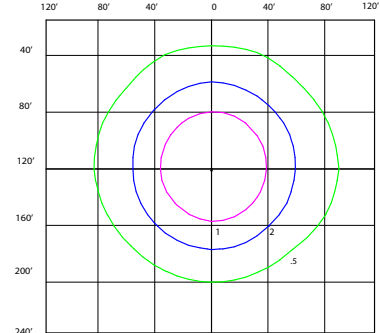
TYPE 5 - 310W 40' MOUNTING HEIGHT
