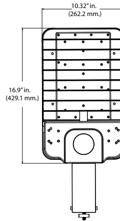
100/145W Model
