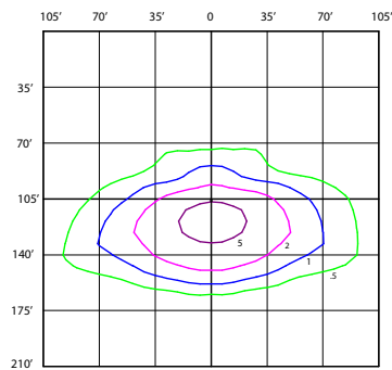
TYPE 3 - 200W 35' MOUNTING HEIGHT
