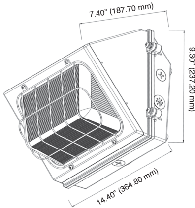
Wire Guard
