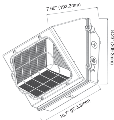
Wire Guard
