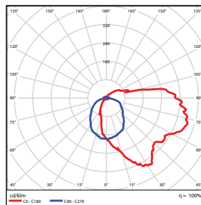
55 Watt DLC Premium
