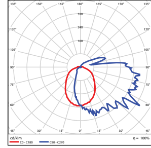
120 Watt DLC Standard
