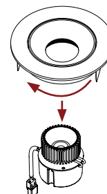
Attach LED module/driver and thread clockwise
