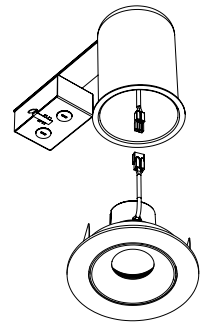
Connect luminaire and install
