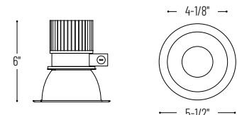
NTG-4SPH 4" Decorative Glass
