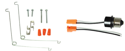
NLOPAC-56RECKIT Retrofit Kit for 5" or 6" Recessed Housings
