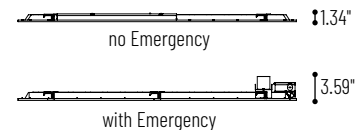
NPDBL-E24 2' x 4' LED Backlit Panel
