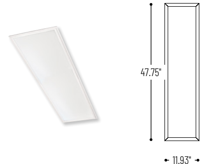
NPDBL-E14 1' x 4' LED Backlit Panel
