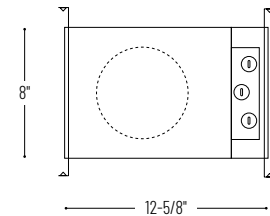
4-3/8" Ceiling Cut-out
