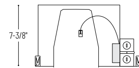
4-3/8" Ceiling Cut-out
