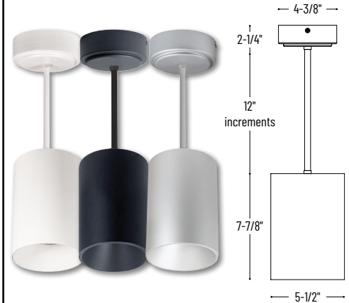
NYLM-5ST Stem Mounted
