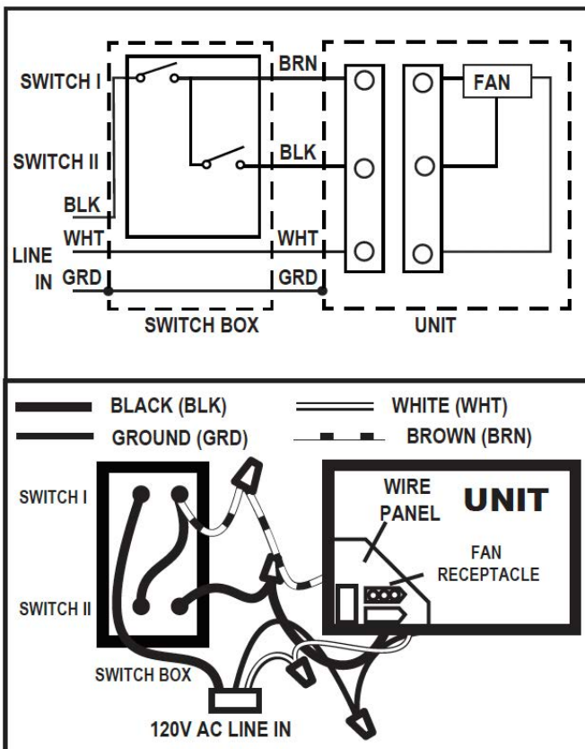
ODD-100HS Wiring Diagram
