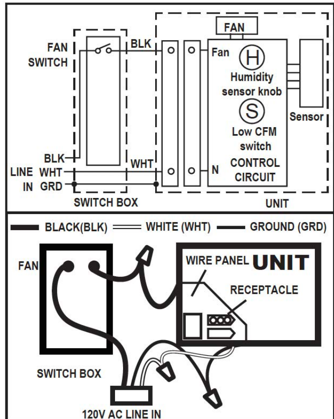
ODD-100HS+MS Wiring Diagram
