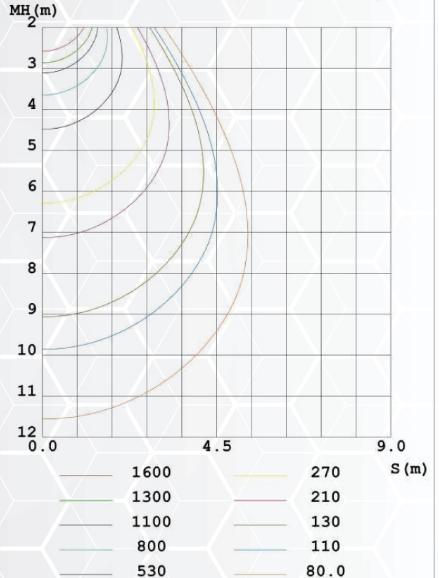
C0 PLANE ISOLUX DIAGRAM (UNIT: lx)
