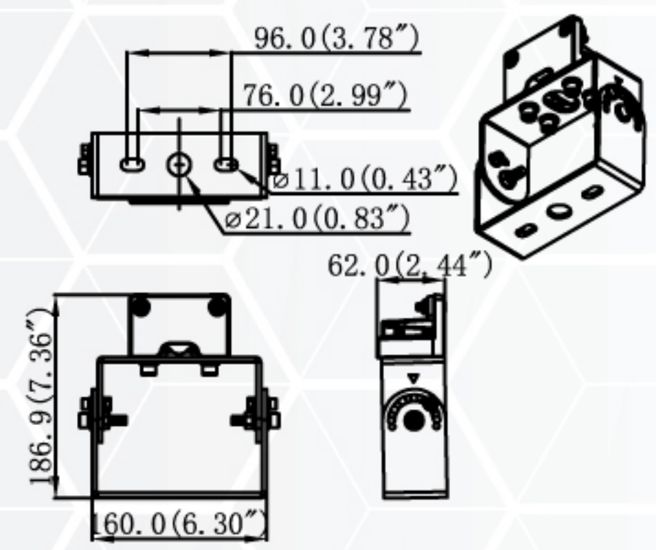
SB-TRUNNION-1 SB-TRUNNION*
