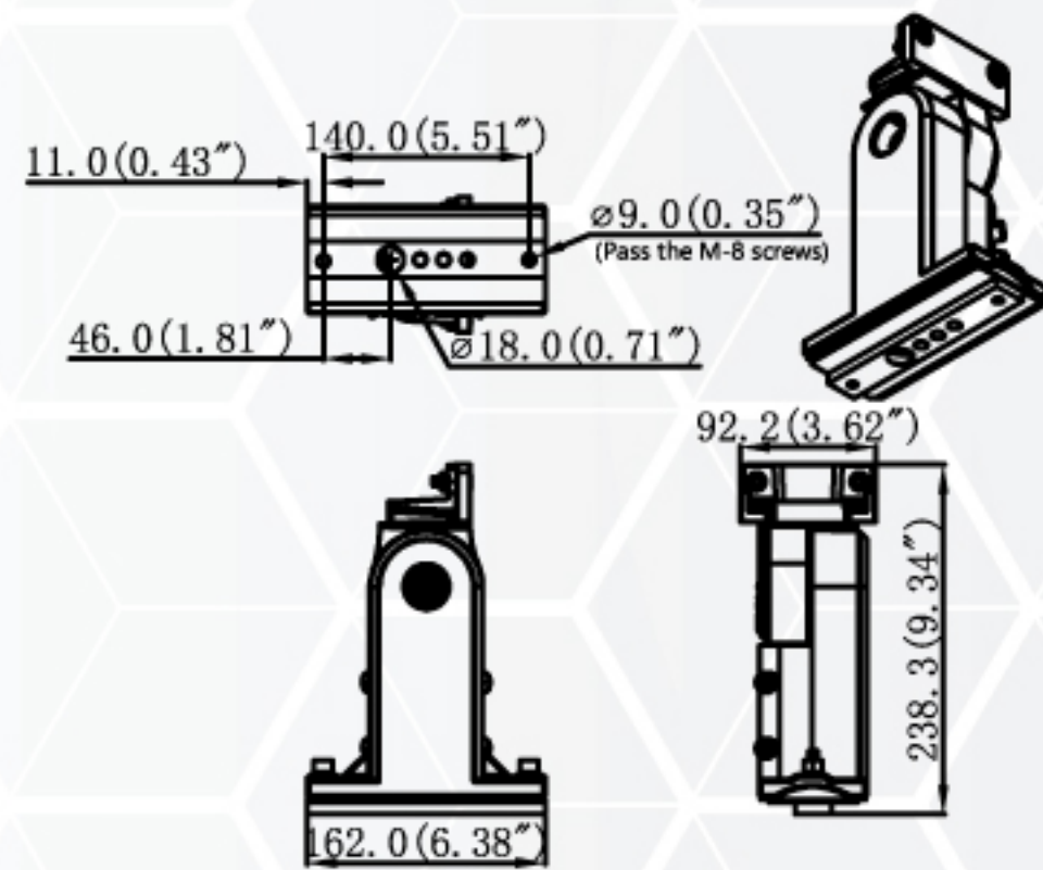
SB-POLE-M1 SB-POLE MOUNT*
