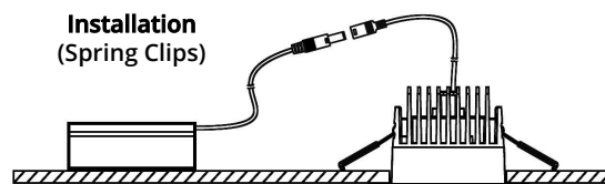
Installation (Spring Clips) Cutout: Ø 3-47/64" (95mm)
