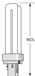
4-Pin Base
